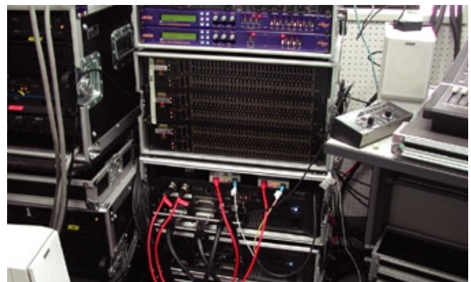
S-4000H with media converter along side of Audio Console
